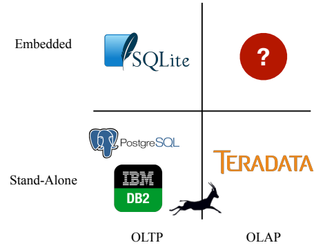
Figure 1: Systems Landscape
